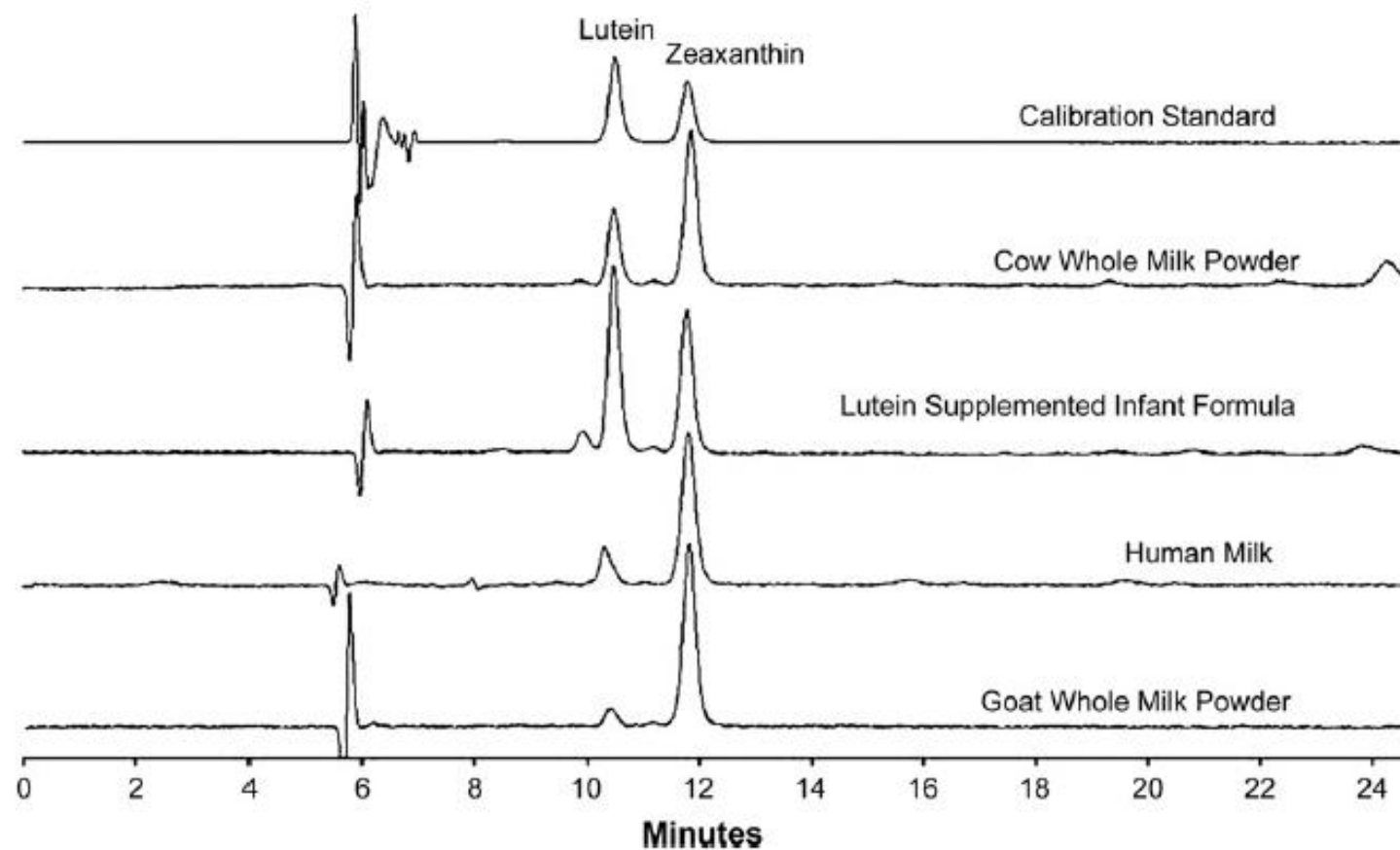
Figure 1. Overlaid chromatograms of milk and powder samples spiked with zeaxanthin internal standard (column: YMC Carotenoid C 30 , 250 × 4.6 mm, 3 μm; mobile phase methanol:dichloromethane (70:30 v/v); flow rate: 0.5 mL min -1 ; detection: 450 nm)
