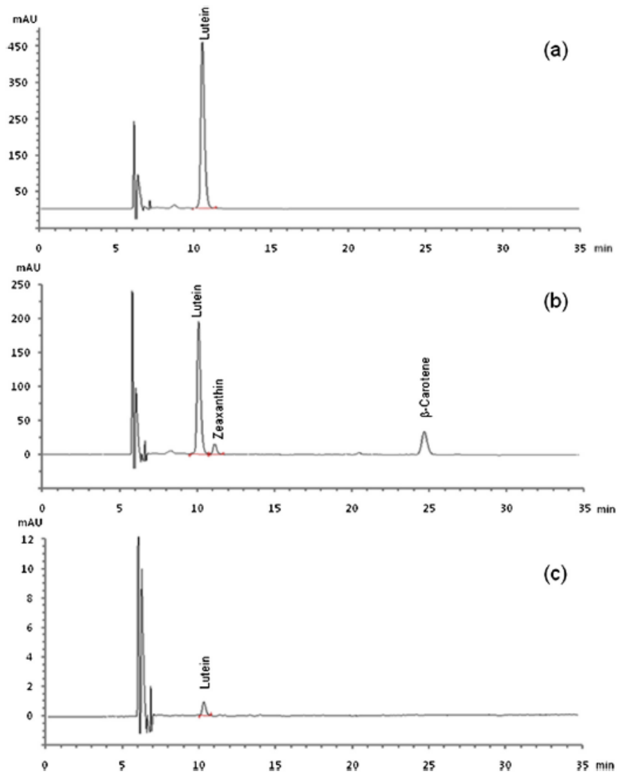
Figure 1. Chromatography obtained under described conditions. Column was YMC C 30 (250 × 4.6 mm, 3 μm); mobile phase, methanol:dichloromethane (70:30, v/v) at 0.5 mL min -1 ; detection, 450 nm. Samples were (a) authentic lutein standard; (b) carotenoid-dosed oil blend; (c) undosed oil blend
