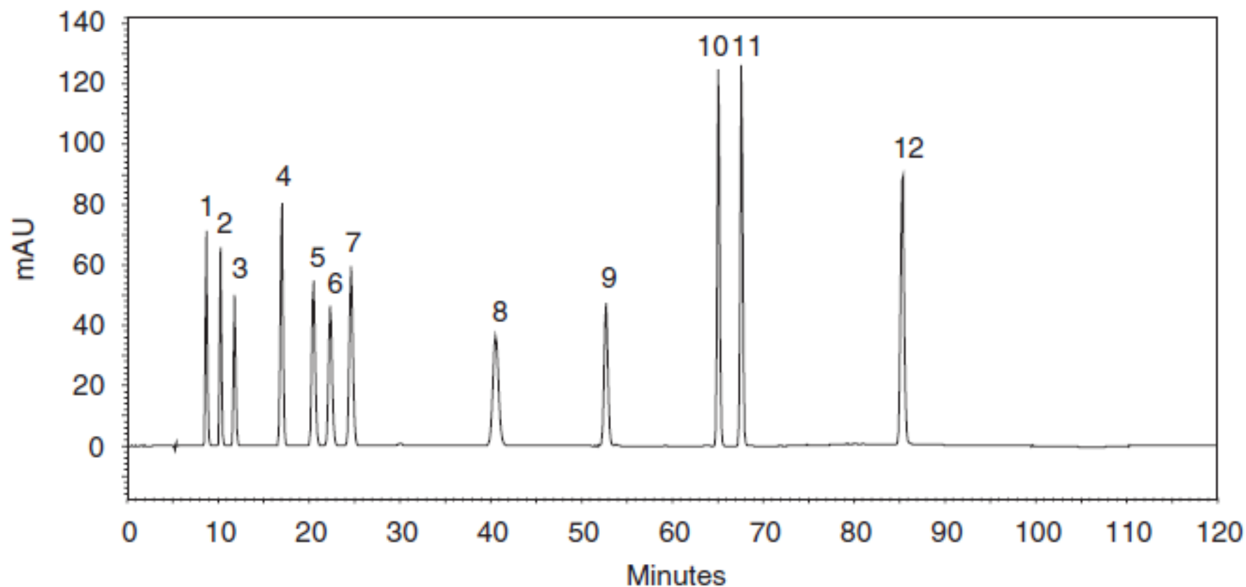
Figure 1. Chromatography of a standard mixture of: (1) 27.8 mM cytidine 5'-monophosphate, (2) 61.9 mM orotic acid, (3) 20.0 mM uridine 5'-monophosphate, (4) 59.7 mM uric acid, (5) 17.9 mM guanosine 5'-monophosphate, (6) 19.4 mM inosine 5'-monophosphate, (7) 44.8 mM cytidine, (8) 37.8 mM uridine, (9) 20.4 mM adenosine 5'-monophosphate, (10) 35.7 mM inosine, (11) 34.8 mM guanosine, (12) 35.9 mM adenosine. Conditions: mobile phase A: \text{KH}_2\text{PO}_4 (0.1 M), pH = 5.6; mobile phase B: \text{KH}_2\text{PO}_4 (0.1M), 15% methanol, pH = 5.6; gradient elution: flowrate 0.5 \text{ mL min}^{-1} throughout, 0–30 min (100% A, 0%B), 65–90 min (0%A, 100%B), 95–130 min (100%A, 0%B). UV detection 260 nm
