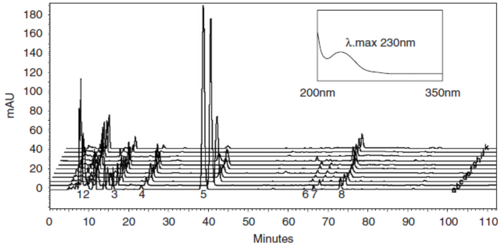
Figure 2. Chromatography of early lactation milk of a single cow: (a–k) 0.3, 0, 0.25, 0.5, 1, 2, 5, 10, 16, 21, 31 days post-partum respectively. (1) cytidine 5'-monophosphate, (2) orotic acid, (3) uric acid, (4) cytidine, (5) uridine, (6) inosine, (7) guanosine, (8) unknown peak (UV spectrum shown in inset). Conditions: mobile phase A: \text{KH}_2\text{PO}_4 (0.1 M), pH = 5.6; mobile phase B: \text{KH}_2\text{PO}_4 (0.1 M), 15% methanol, pH = 5.6; gradient elution: flow rate 0.5 \text{ mL min}^{-1} throughout, 0–30 min (100%A, 0%B), 65–90 min (0%A, 100%B), 95–130 min (100%A, 0%B). UV detection 260 nm
